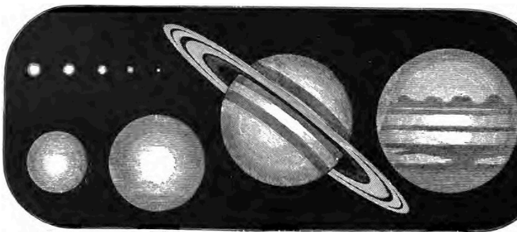
Comparative Size of Planets
